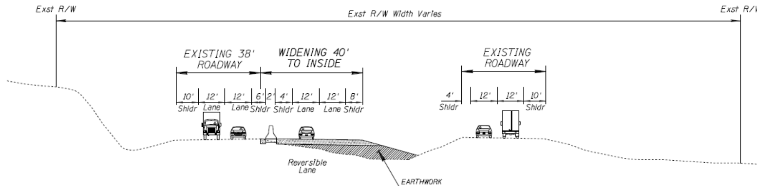
I-17 Typical Section Reversible 2 Lane Alternative
