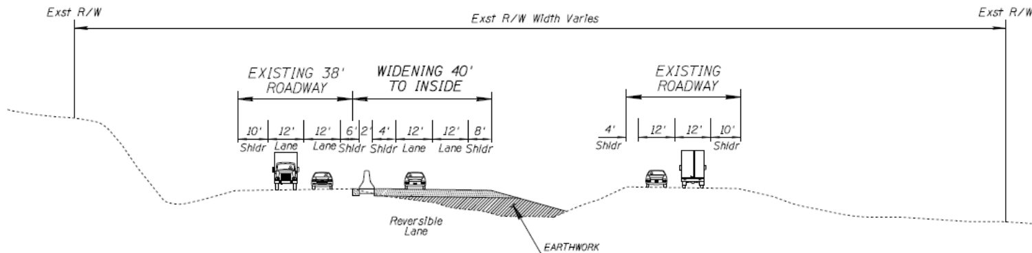
I-17 Typical Section Reversible 2 Lane Alternative
